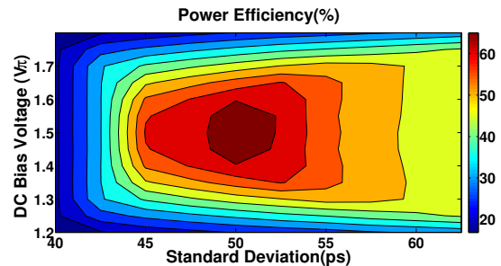
Fig. 4: Power efficiency versus pulse shaping factor and DC biasing voltage.
